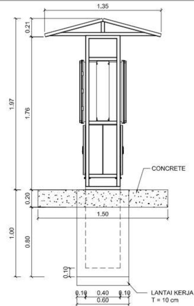
TAMPAK SAMPING
