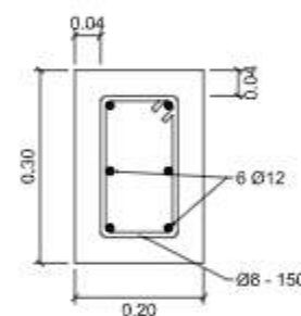
DETAIL SLOOF SKALA 1 : 25
