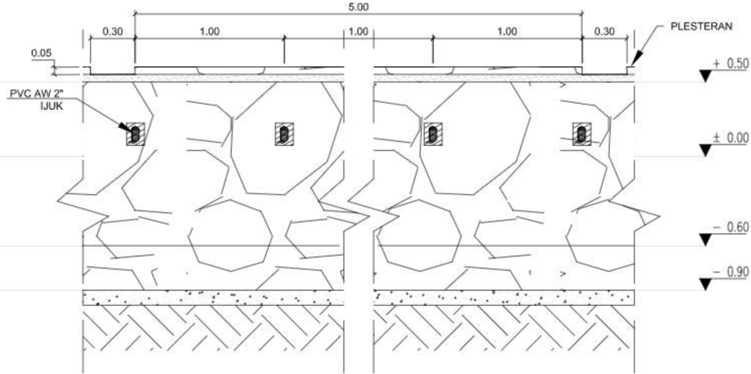
DETAIL PIPA DPT
