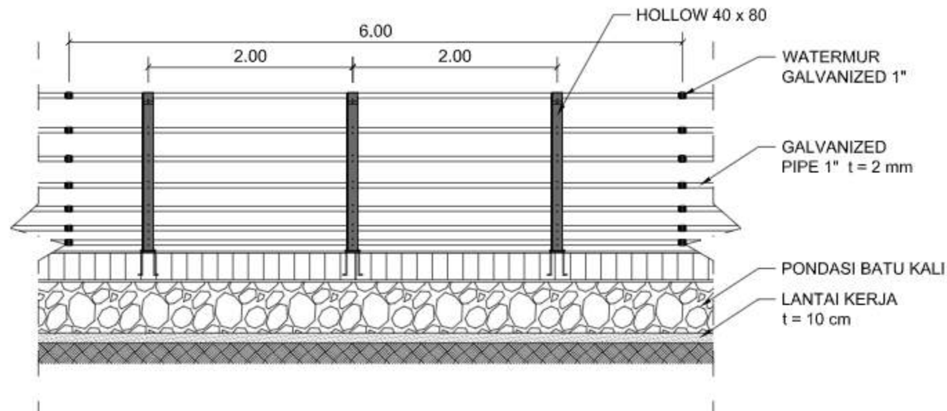
DETAIL DINDING KOLAM SKALA 1 : 100
