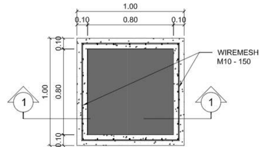
DENAH MANHOLE SKALA 1 : 25
