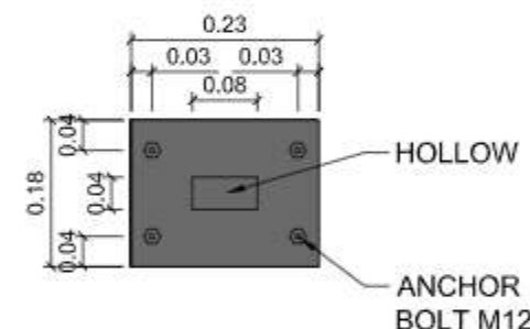
DETAIL BASE PLATE SKALA 1 : 50
