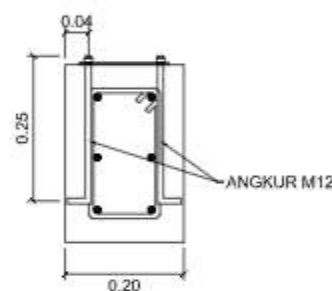
DETAIL ANGKUR SKALA 1 : 25
