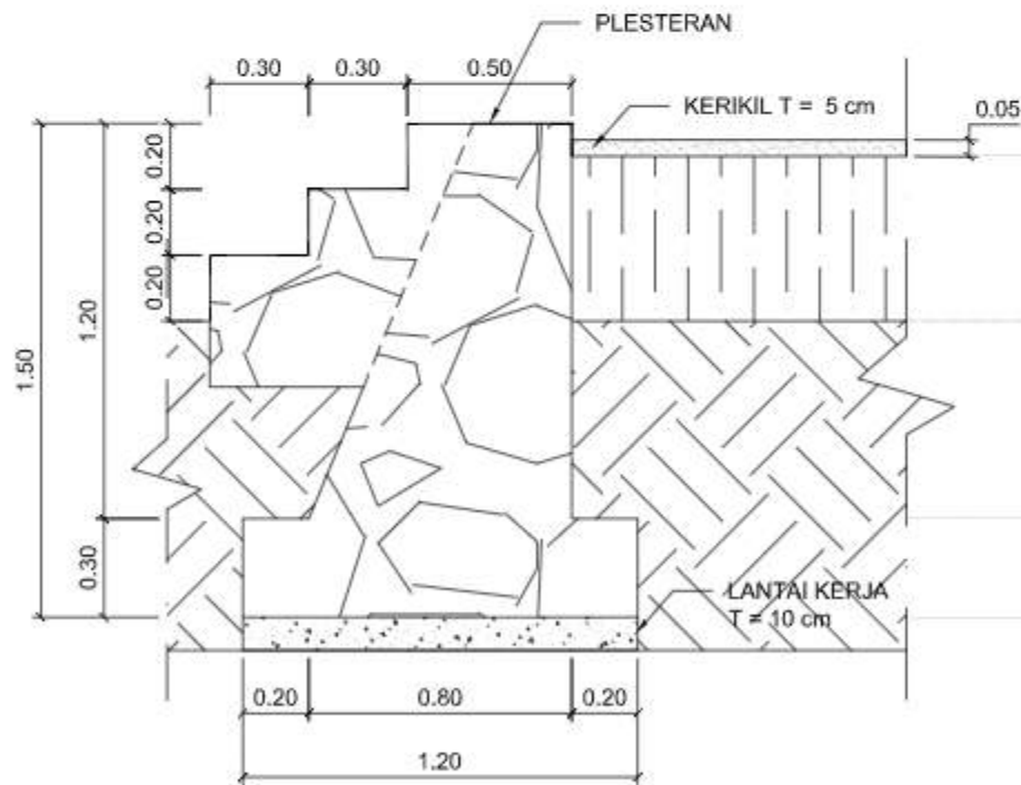
DETAIL DPT KOLAM
