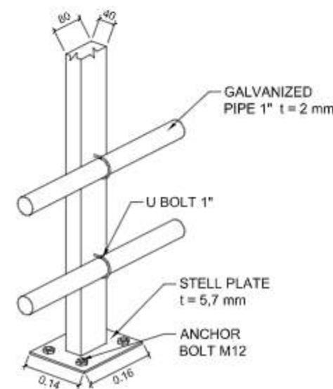
DETAIL ISOMETRI TIANG KOLAM SKALA 1 : 50
