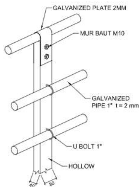
DETAIL ISOMETRI TIANG KOLAM SKALA 1 : 50
