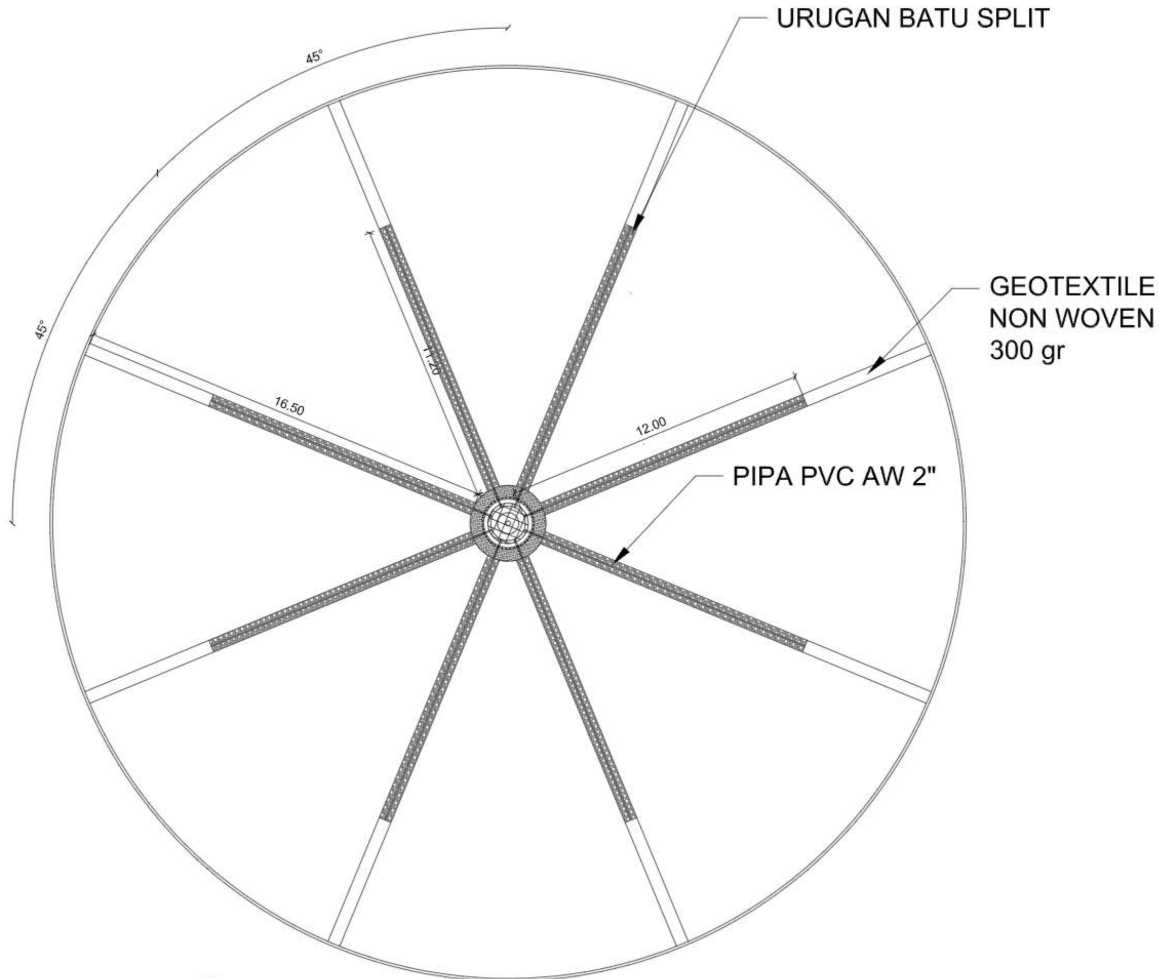
DENAH RESAPAN KOLAM
