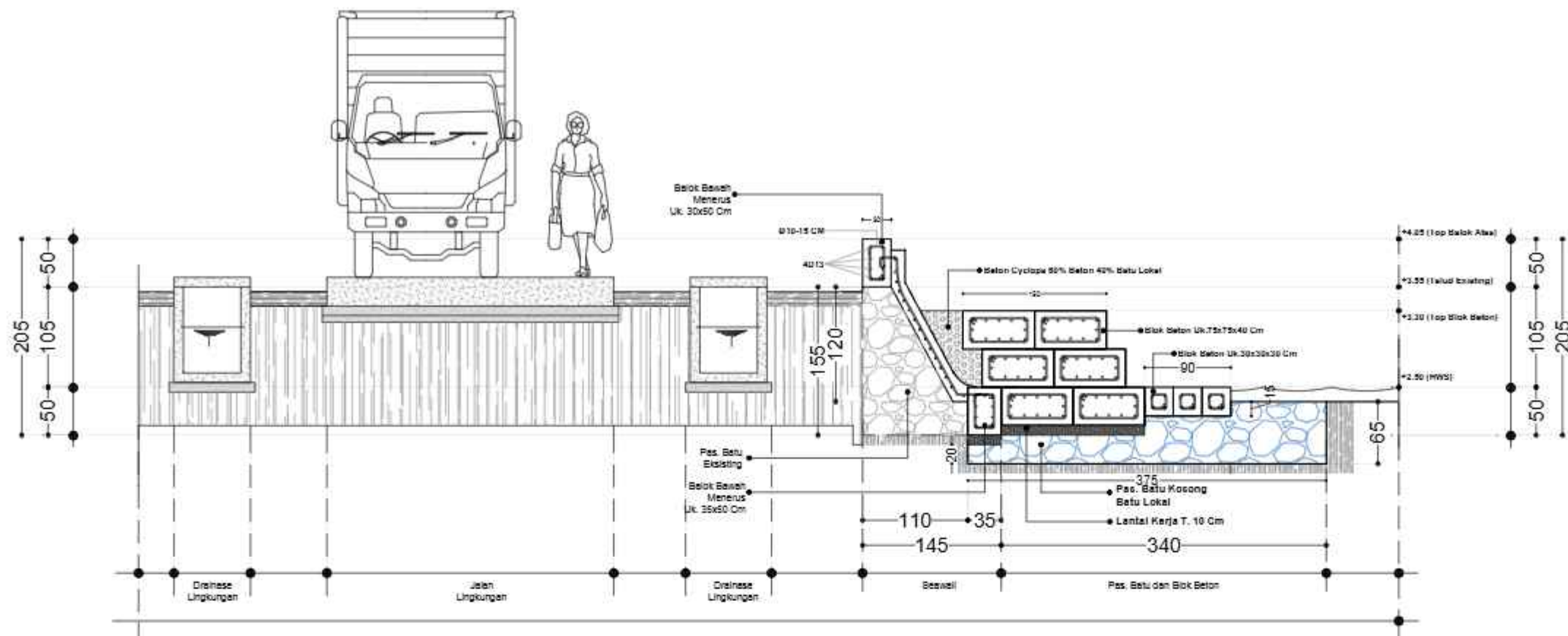
SEGMENT POT. A
