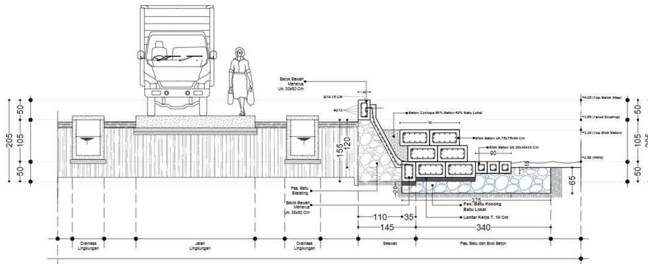
SEGMENT POT. L
