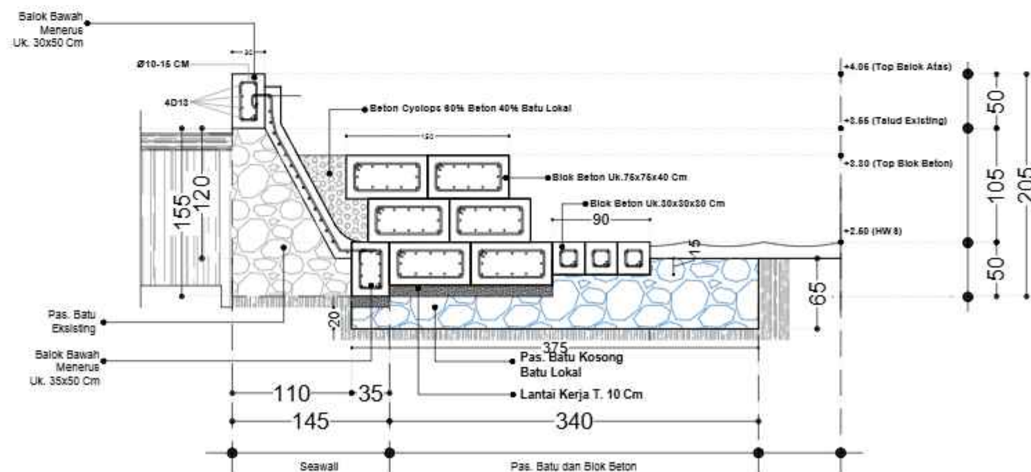
SEGMENT POT. N
