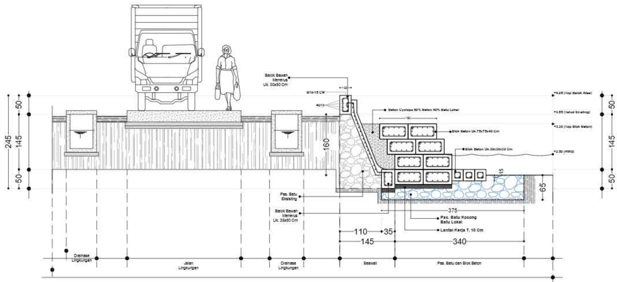
SEGMENT POT. H
