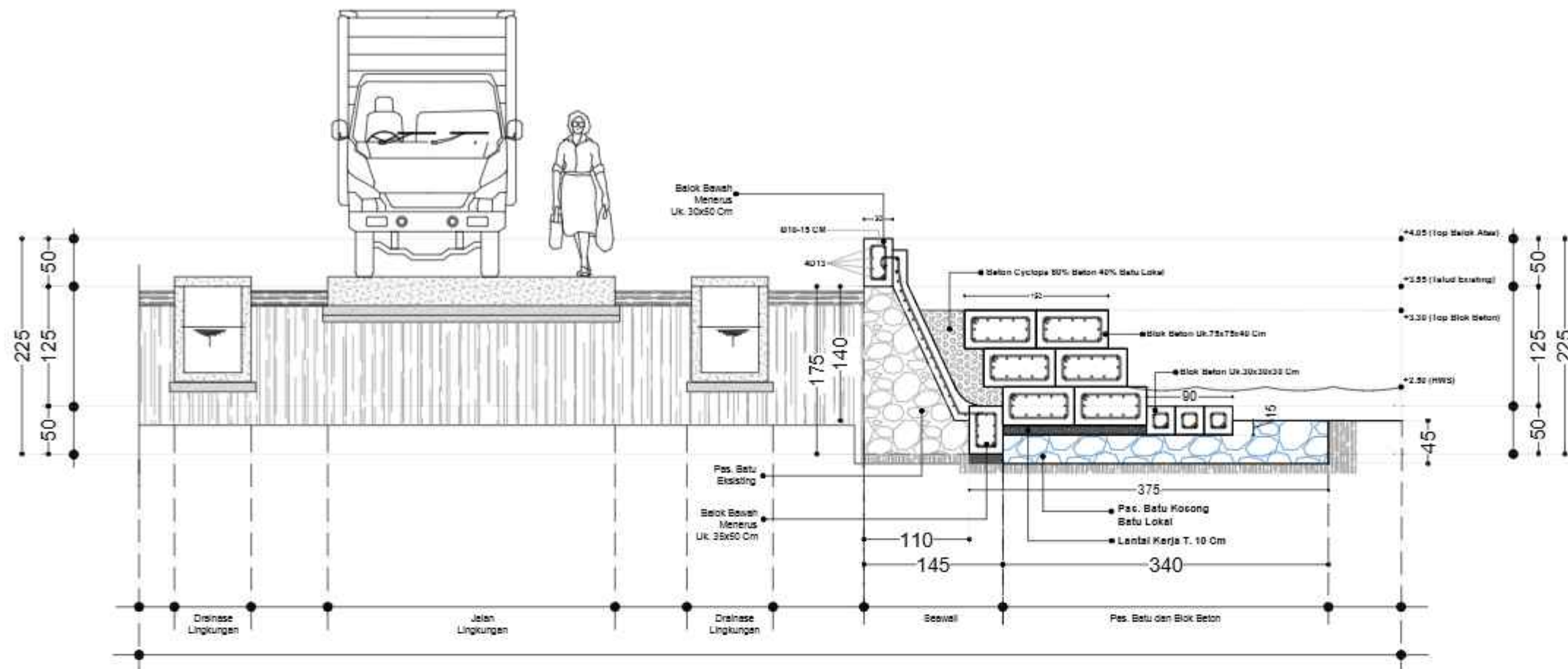
SEGMENT POT. I
