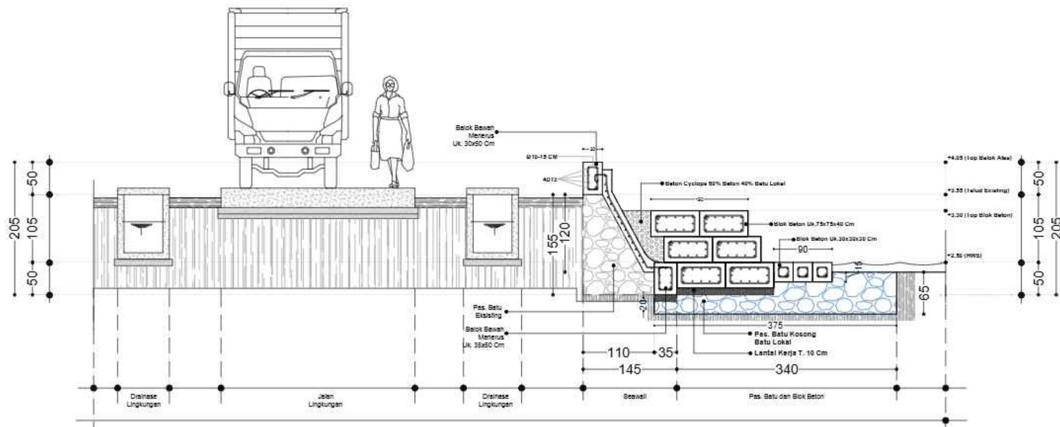
SEGMENT POT. B
