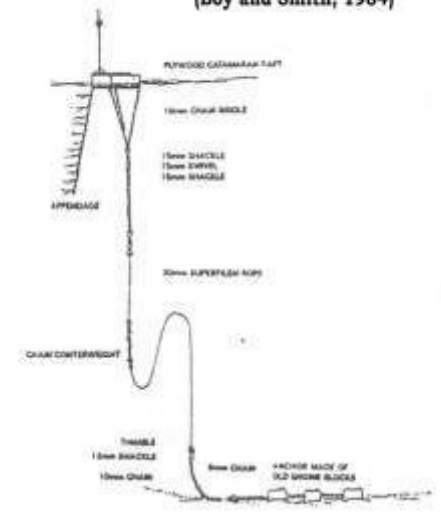
Gambar 22. Payoas Type Vanuatu (Boy and Smith, 1984)
