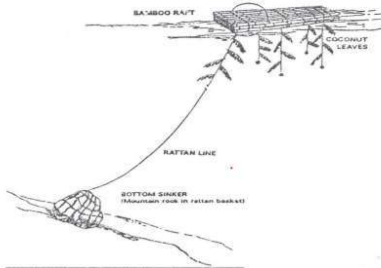
Gambar 20. Payaos Tradisional Selatan Sulawesi (Nasution dll, 1986)
