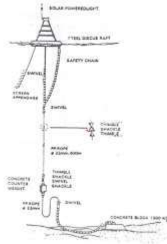
Gambar 19. Payoas Kep. Polynesia (Boy and Smith, 1984)
