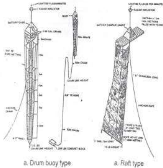
Gambar 15. Payoas Kep. Hawaii (Matsumoto dll, 1981)
