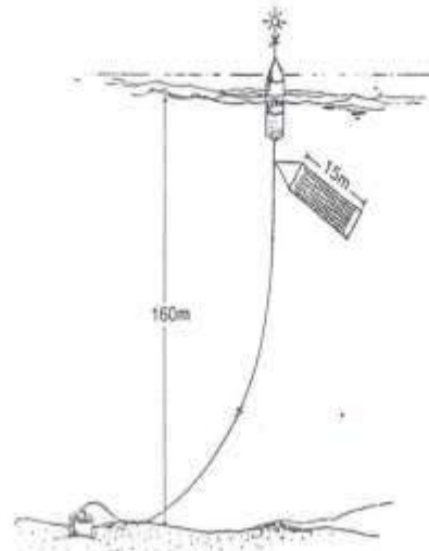
Gambar 16. Rumpon Type Australia
